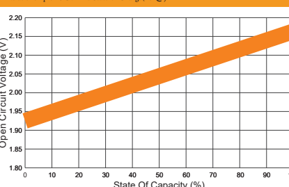
Relationship of OCV And State of Charge(20°C)
