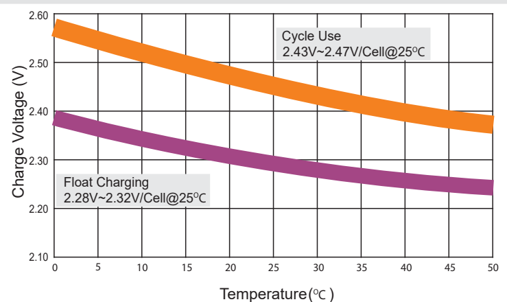
Relationship Between Charging Voltage And Temperature
