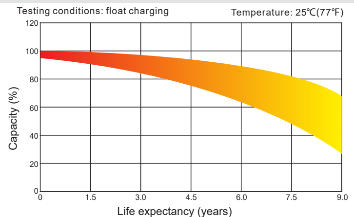
Life Characteristics Of Standby Use
