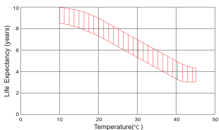
Effect Of Temperature On Long Term Life
