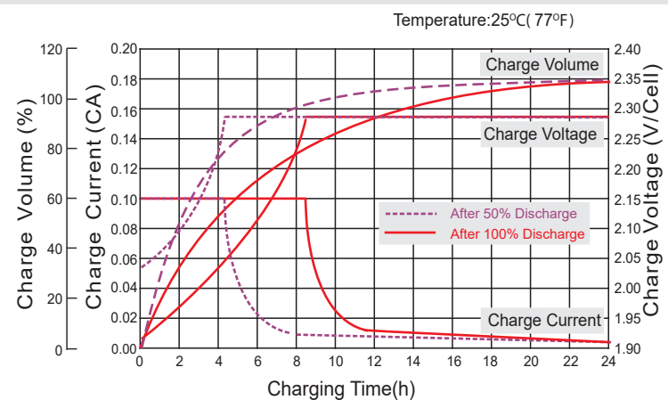
Charge Characteristic Curve For Standby Use(IU)
