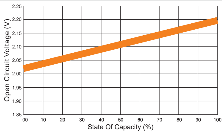
Relationship of OCV And State of Charge(20°C)
